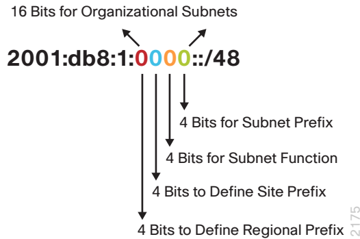
Figure 16 - Subnet breakdown
