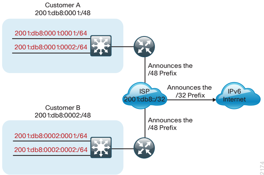
Figure 11 - Hierarchical addressing
