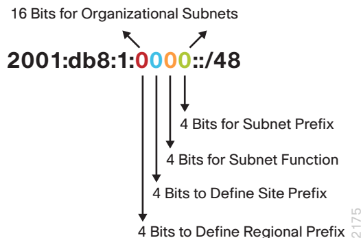
Figure 12 - Prefix breakdown
