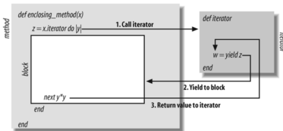
Figure 5-4. The next statement in a block
