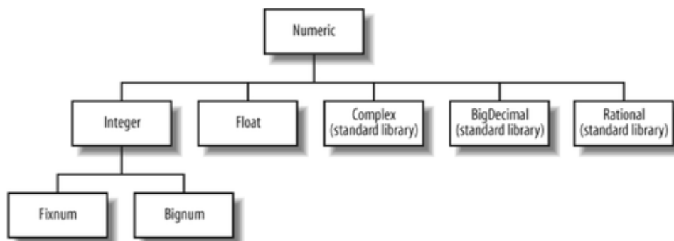
Figure 3-1. Numeric class hierarchy
