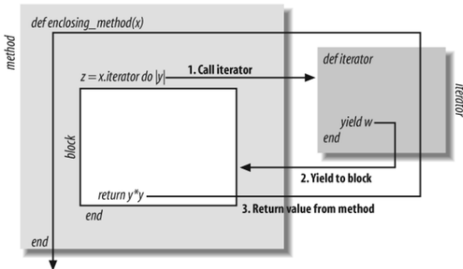
Figure 5-2. The return statement in a block
