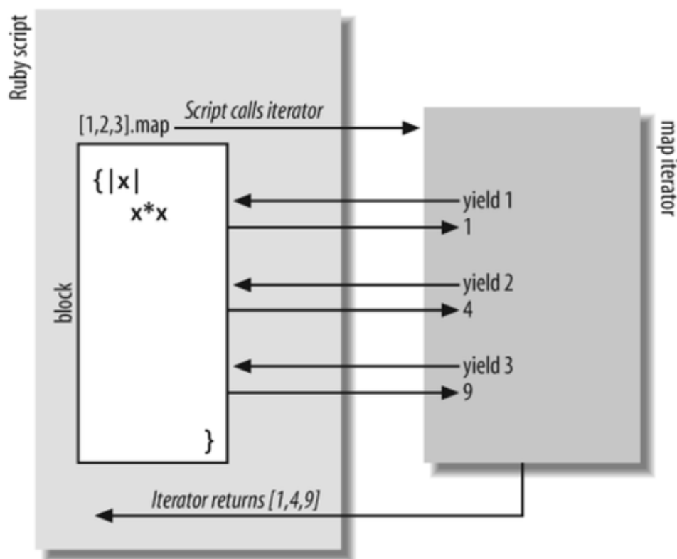
Figure 5-1. An iterator yielding to its invoking method
